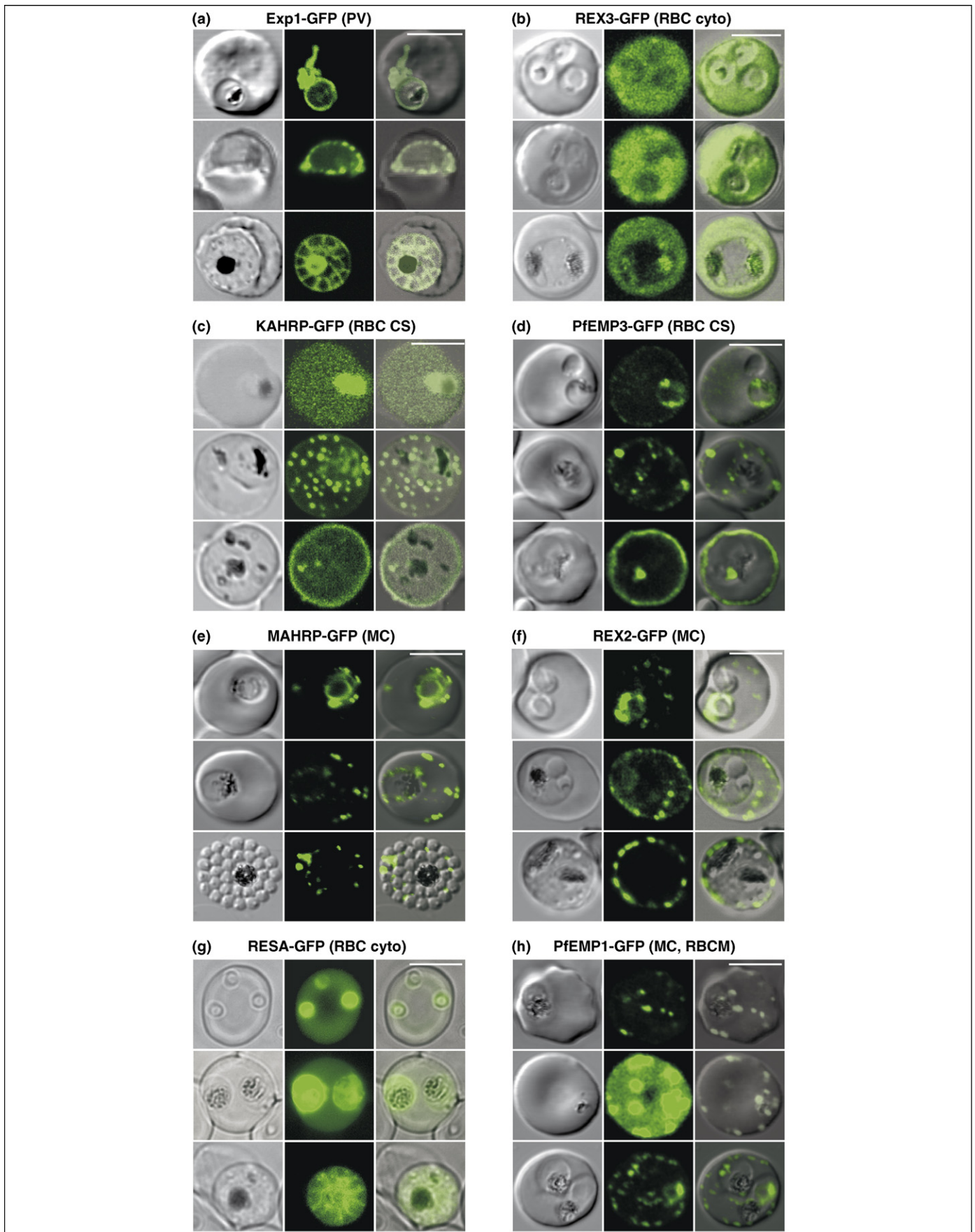
Figure 2. Transfected Plasmodium falciparum -infected RBCs expressing GFP chimeras directed to compartments within the host cytoplasm. The images represent a DIC image, the GFP fluorescence signal and an overlay of these images. (a) Exp 1-35 -GFP transfectant (PV). Some ring and trophozoite stage parasites show a 'necklace of beads' pattern, whereas some parasites show distortions and evaginations of the PV to form a TVN. Schizonts show a segmented pattern with a highly fluorescent central
