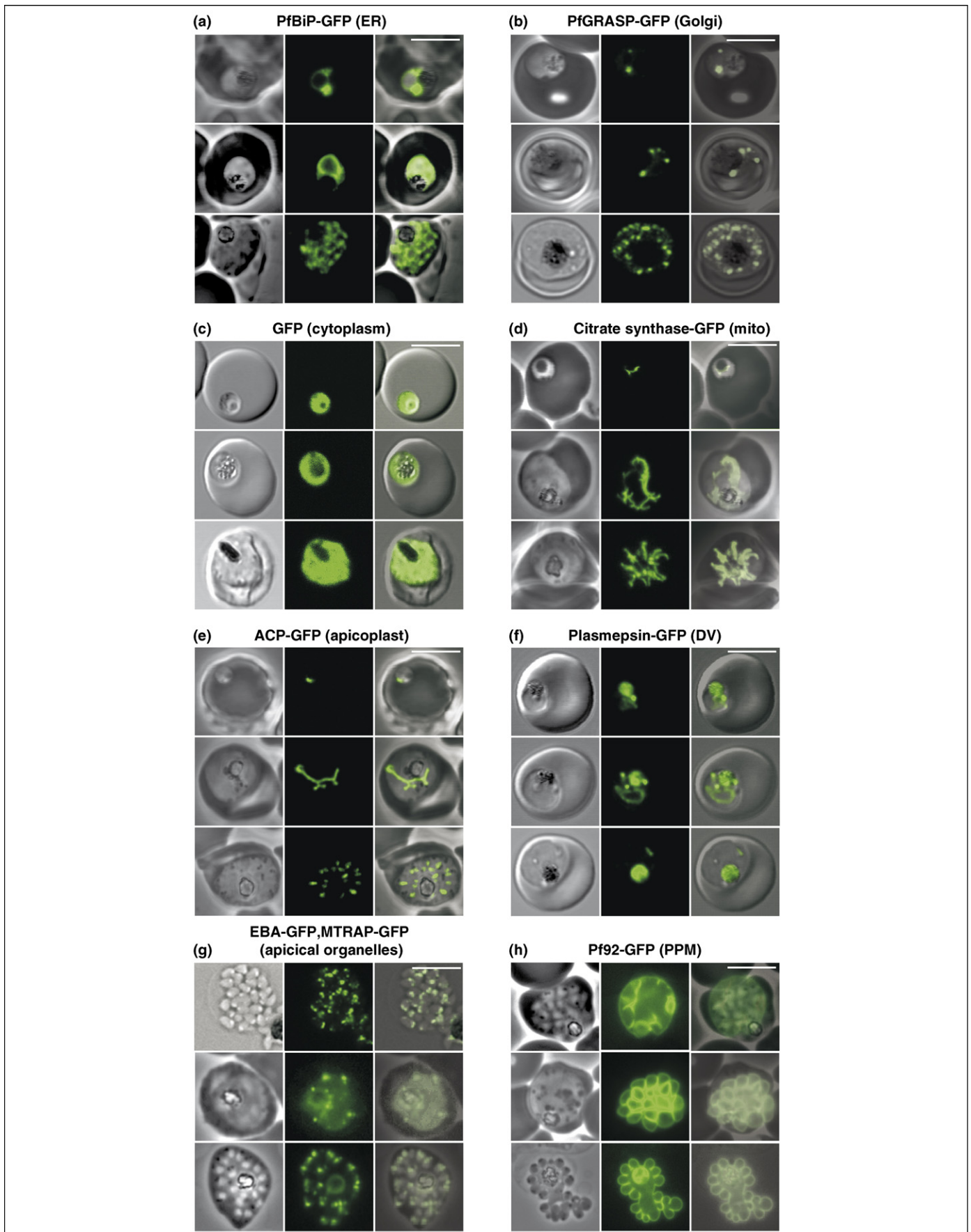
Figure 1. Transfected Plasmodium falciparum -infected RBCs expressing GFP chimeras directed to compartments within the parasite. The images represent a differential interference contrast (DIC) or phase image, the fluorescent protein signal and an overlay of these images. Where possible, early-, mid- and late-stage parasites are shown. (a) PfBiP-GFP transfectant (ER). Ring and early trophozoite stage parasites show a perinuclear ring of fluorescence in the parasite cytoplasm. Schizont stage parasites show
