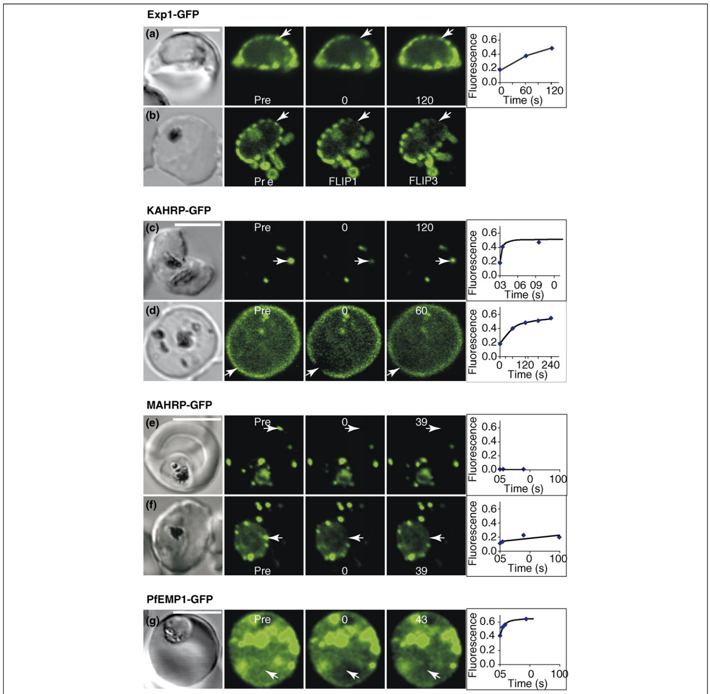
Figure 3. Analysis of the molecular organization of GFP chimeras in transfected Plasmodium falciparum -infected RBCs using fluorescence photobleaching. In each case, the first panel shows the DIC image. The fluorescence images (green) comprise prebleach (pre) and postbleach images at the times (seconds) indicated following the bleach pulse or the fluorescence loss in photobleaching (FLIP) images after repeated bleaching. The position of the bleach pulse is indicated by white arrows. The graphs show the recovery of fluorescence intensity over time in the bleached region relative to the prebleach level. (a) Trophozoite-stage Exp1 1-35 -GFP transfectant showing a 'necklace of beads' fluorescence pattern. A high intensity laser pulse was applied. Partial recovery into this region was observed over two minutes indicating partial connectivity to surrounding regions. (b) Exp1 1-35 -GFP transfectant subject to FLIP analysis. The region indicated by the arrow was repeatedly subjected to an intense laser pulse. Loss of fluorescence was restricted to regions near the bleach spot, which indicated connectivity between adjacent 'beads' but no connectivity to distal compartments. (c) KAHRP 1-123 -GFP transfectant. The fluorescence associated with a Maurer's cleft was ablated. (d) KAHRP 1-123 -GFP transfectant. Fluorescence associated with a region of the RBC membrane was ablated. Some recovery of the fluorescence was observed because of exchange between cytoplasmic and bound pools of the chimera. (e) Bleaching of MAHRP1-GFP in a tethered peripheral Maurer's cleft. (f) Bleaching of MAHRP1-GFP in a PV membrane-associated focal region (nascent Maurer's cleft). There is no recovery of the signal, which indicates that the Maurer's clefts are physically separate structures. (g) A KAHRP 118 -PfEMP1-TM-C-term-GFP transfectant was imaged at high photomultiplier gain to visualize the faint fluorescence in the RBC cytoplasm. A region of the cytoplasm was subjected to a bleach pulse and recovery was observed over several seconds. The data are consistent with the presence of large complexes of the chimera in the RBC cytoplasm. Scale bar = 5 \mu m.
