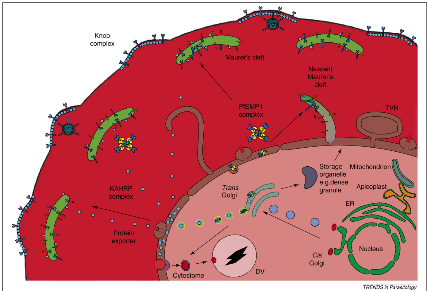
Figure 4. Diagrammatic representation of some putative trafficking pathways in a Plasmodium falciparum -infected RBC delineated using GFP transfectants. Soluble proteins destined for export are directed into the ER and pass through exit sites to a closely apposed cis -Golgi, then to a more distal trans -Golgi en route to the PV. Some proteins are retrieved from the PM or diverted from the ER or Golgi to intracellular organelles such as the DV and the apicoplast or (in the schizont stage) to regulated secretory compartments such as the dense granules, rhoptries and micronemes. Some proteins destined for locations beyond the PV membrane are first released into the PV. Recognition of a PEXEL motif enables translocation of proteins across the PV membrane. Exported soluble proteins can form complexes as they diffuse across the RBC cytosol and might interact with the cytoplasmic surface of the Maurer's clefts before redistribution to the RBC membrane skeleton. Some exported integral membrane proteins, such as PfEMP1, seem to be trafficked through the same PEXEL recognition machinery. The Maurer's clefts contain resident proteins, such as MAHRP1, that accumulate in these structures as they form. PfEMP1 might cross the RBC cytoplasm as a protein complex or might be inserted into nascent Maurer's clefts. The Maurer's clefts seem to bud from the PV membrane and form separate structures tethered to the RBC membrane. Some exported proteins lack a recognizable PEXEL motif and could use alternative pathways.
